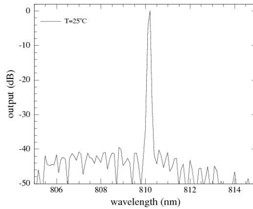
Room Temperature CW Spectrum at 810nm
