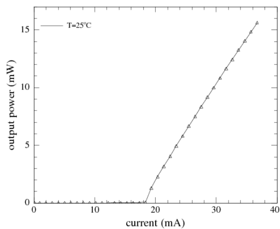
Power against Operating Current
